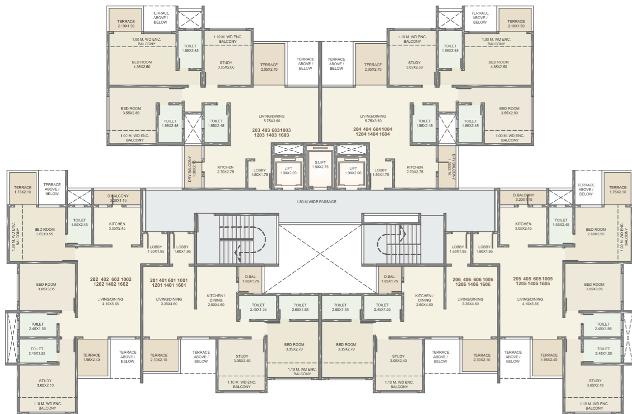
M Building Even Floor Plan 2nd, 4th, 6th, 10th, 12th, 14th, 16th Floor Plan
