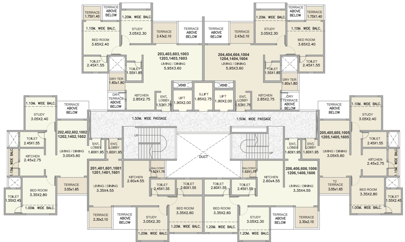
K Building Even Floor Plan 2nd, 4th, 6th, 8th, 10th, 14th, 16th Floor Plan
