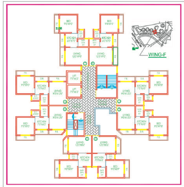
2ND TO 6TH, 7TH & 9TH FLOOR
