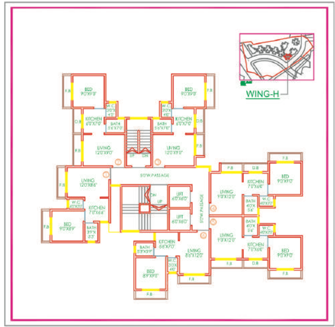
2ND TO 6TH, 7TH & 9TH FLOOR
