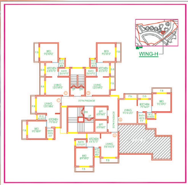
EIGHTH FLOOR PLAN (REFUGE FLOOR)
