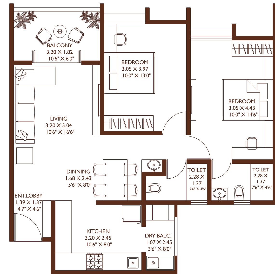
2BHK - Type 2
