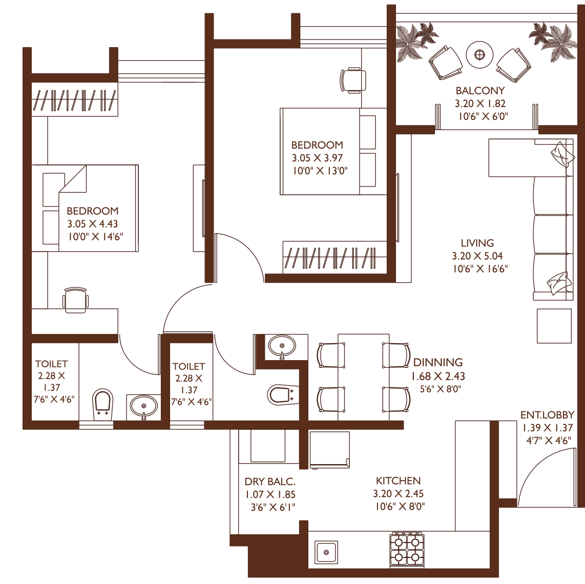
2BHK - Type 3
