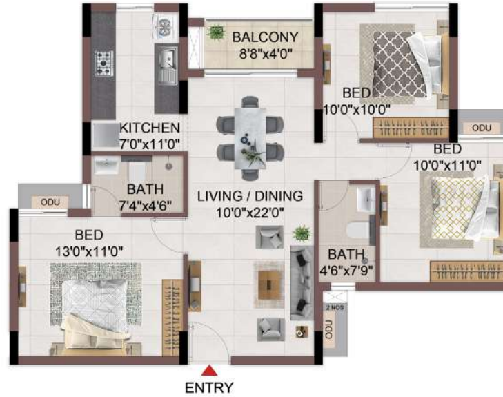
TYPICAL FLOOR 1ST TO 4TH
