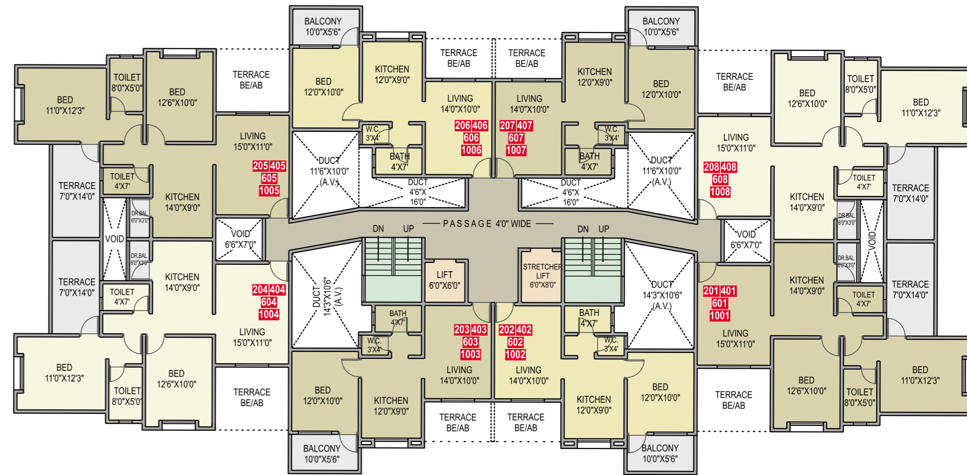
SECOND / FOURTH / SIXTH / TENTH FLOOR PLAN
