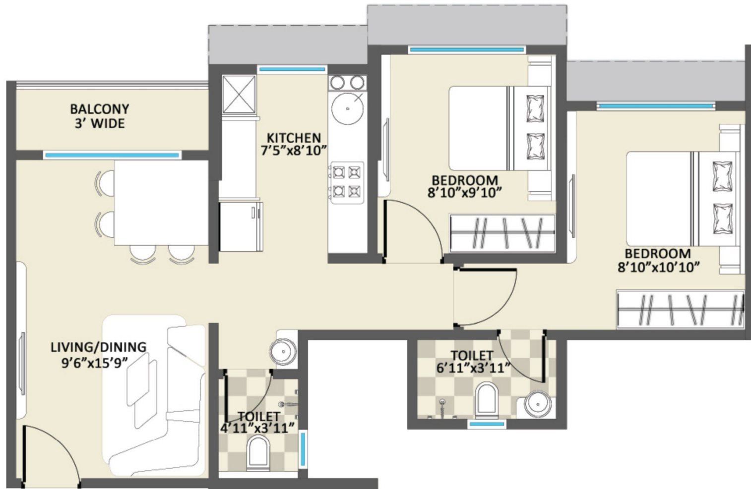
2BHK UNIT PLAN
