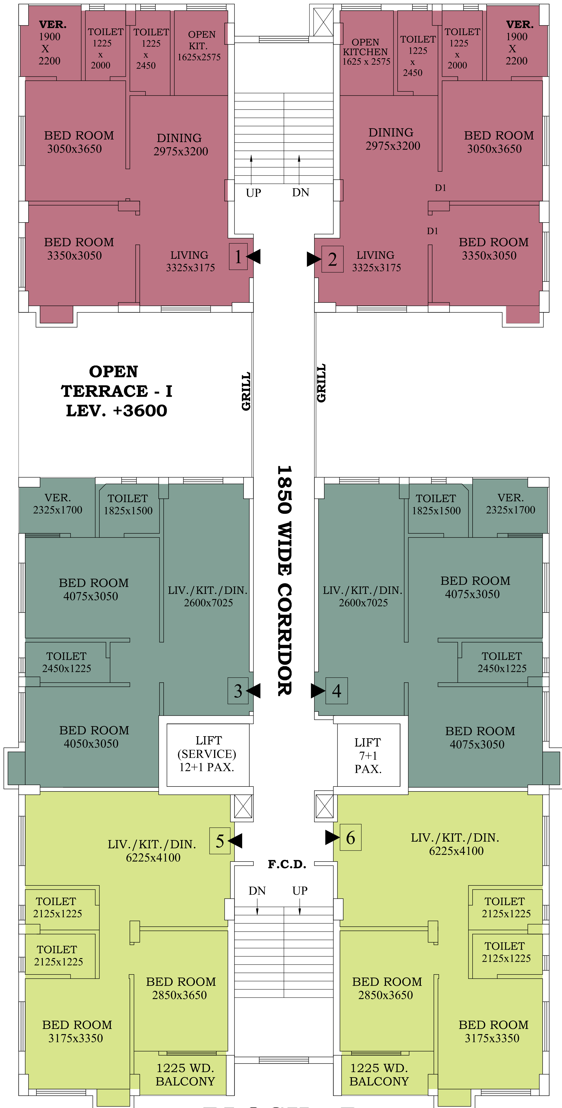
BLOCK - B TYPICAL FLOOR PLAN
