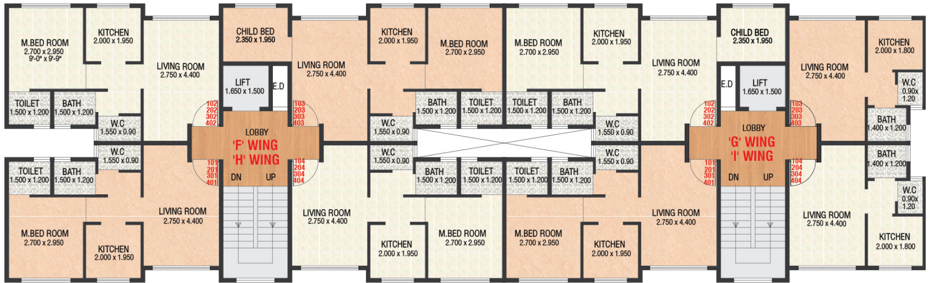
Typ. 1st to 4th Floor Plan (BLDG.F-G-H-I)
