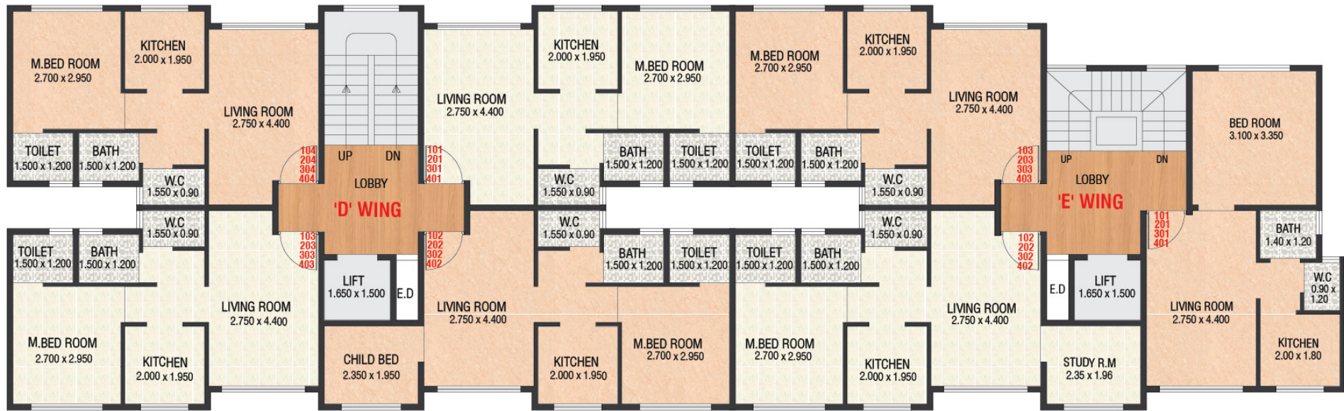
Typ. 1st to 4th Floor Plan (BLDG.D-E)
