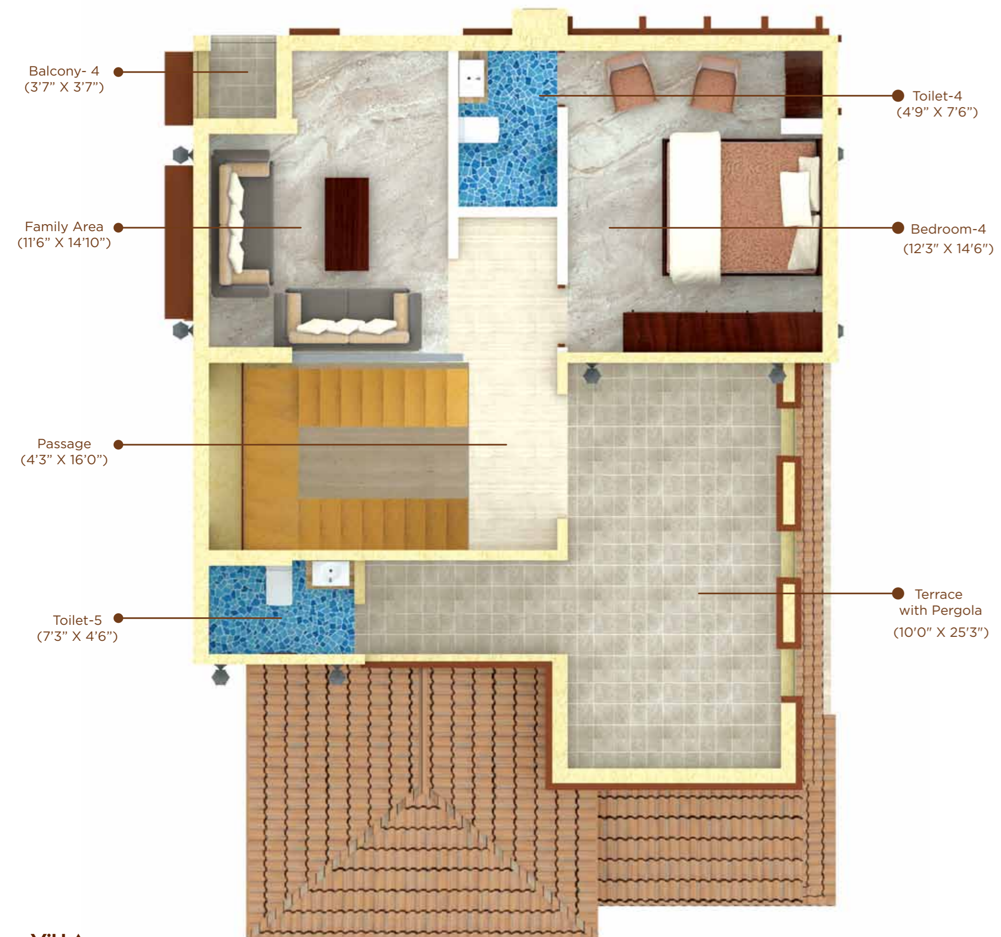
VILLA: SECOND FLOOR PLAN
