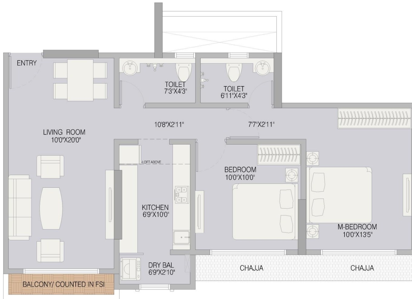
WING-B & C 2 BHK UNIT PLAN-1
