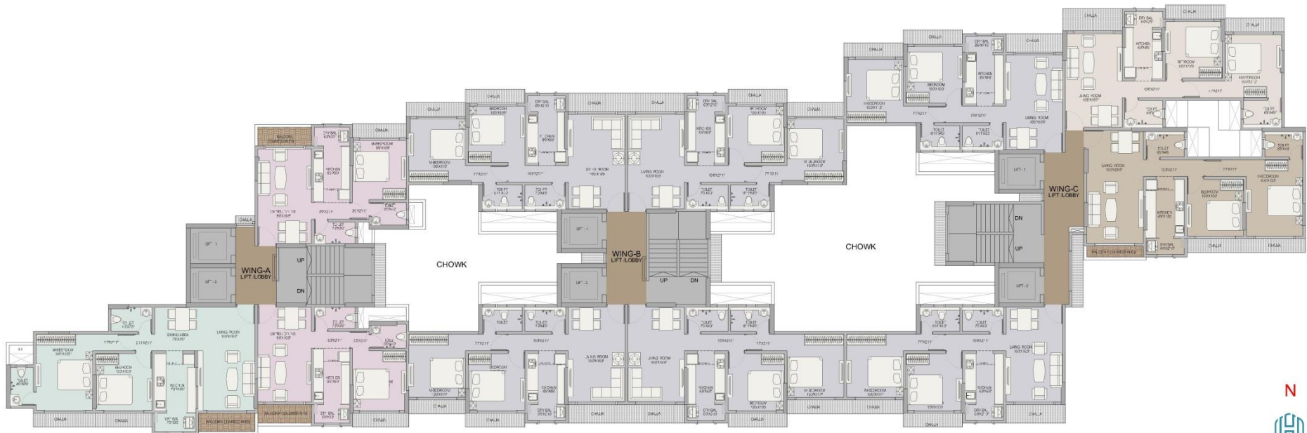
11TH FLOOR PLAN
