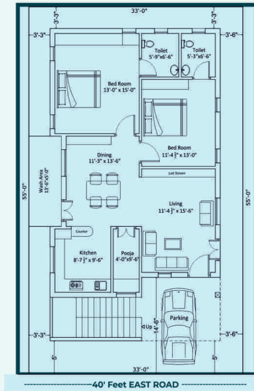
GROUND FLOOR PLAN 1227.00 SQ FTS SLAB AREA 1069.00 SQ FTS PLINTH AREA
