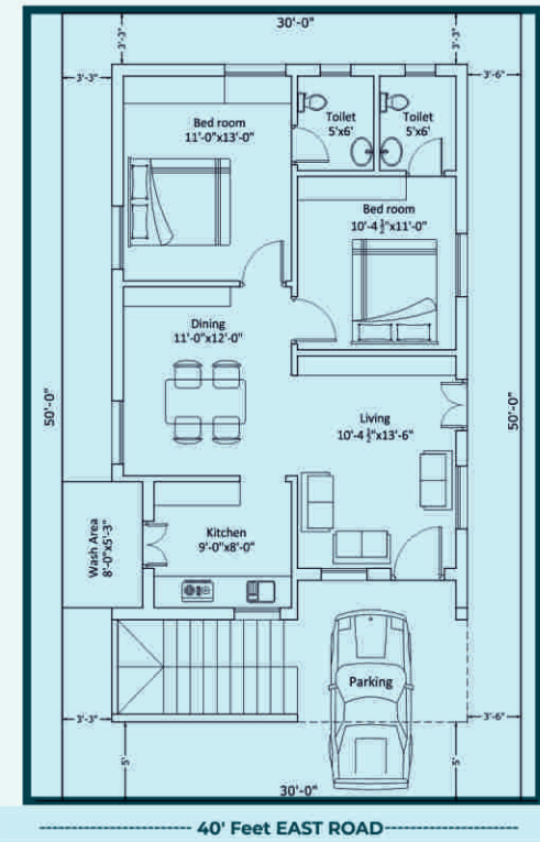
GROUND FLOOR PLAN 970.00 SQ FTS SLAB AREA 820.00 SQ FTS PLINTH AREA
