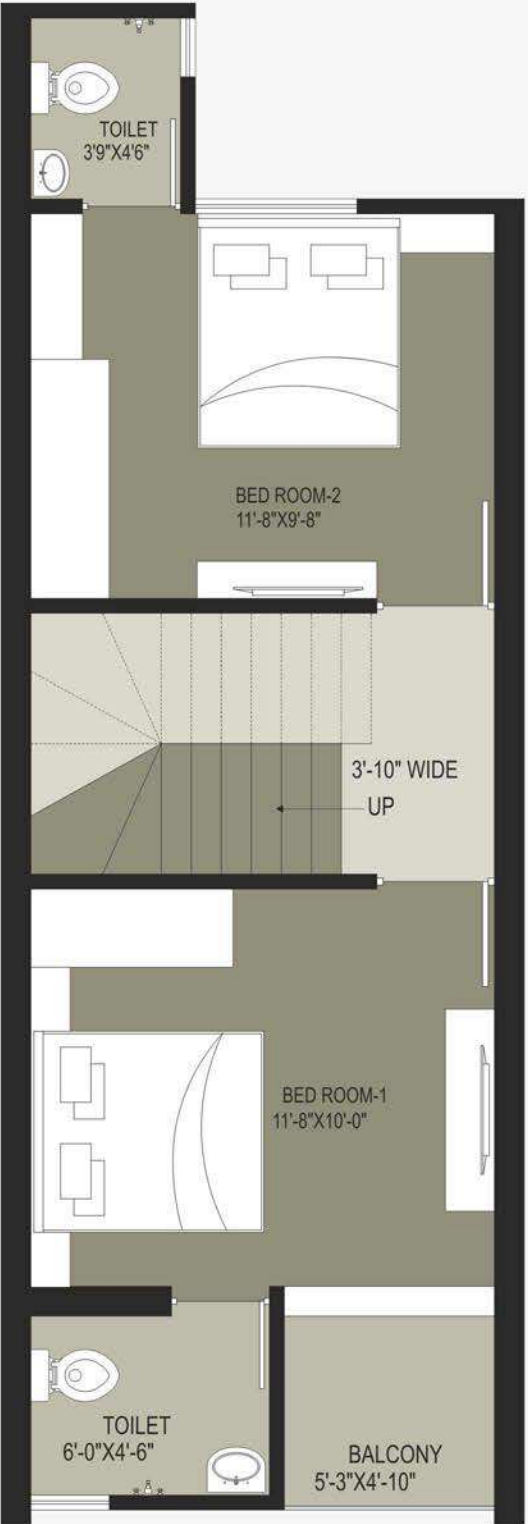
FIRST FLOOR
