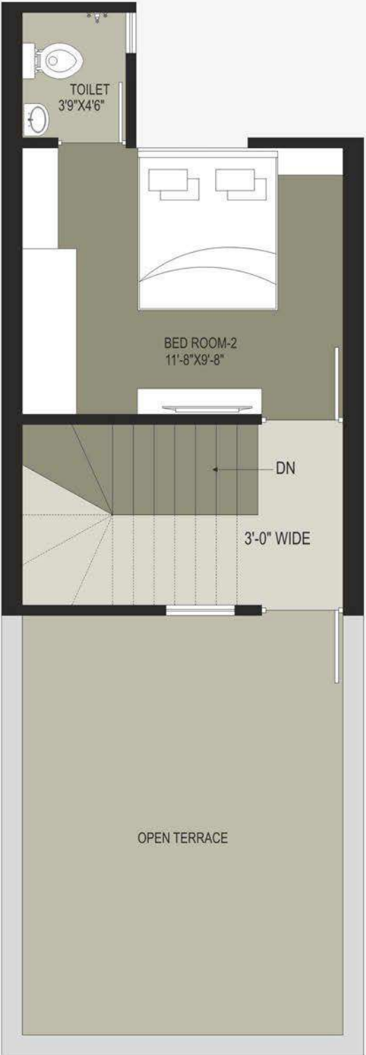
SECOND FLOOR
