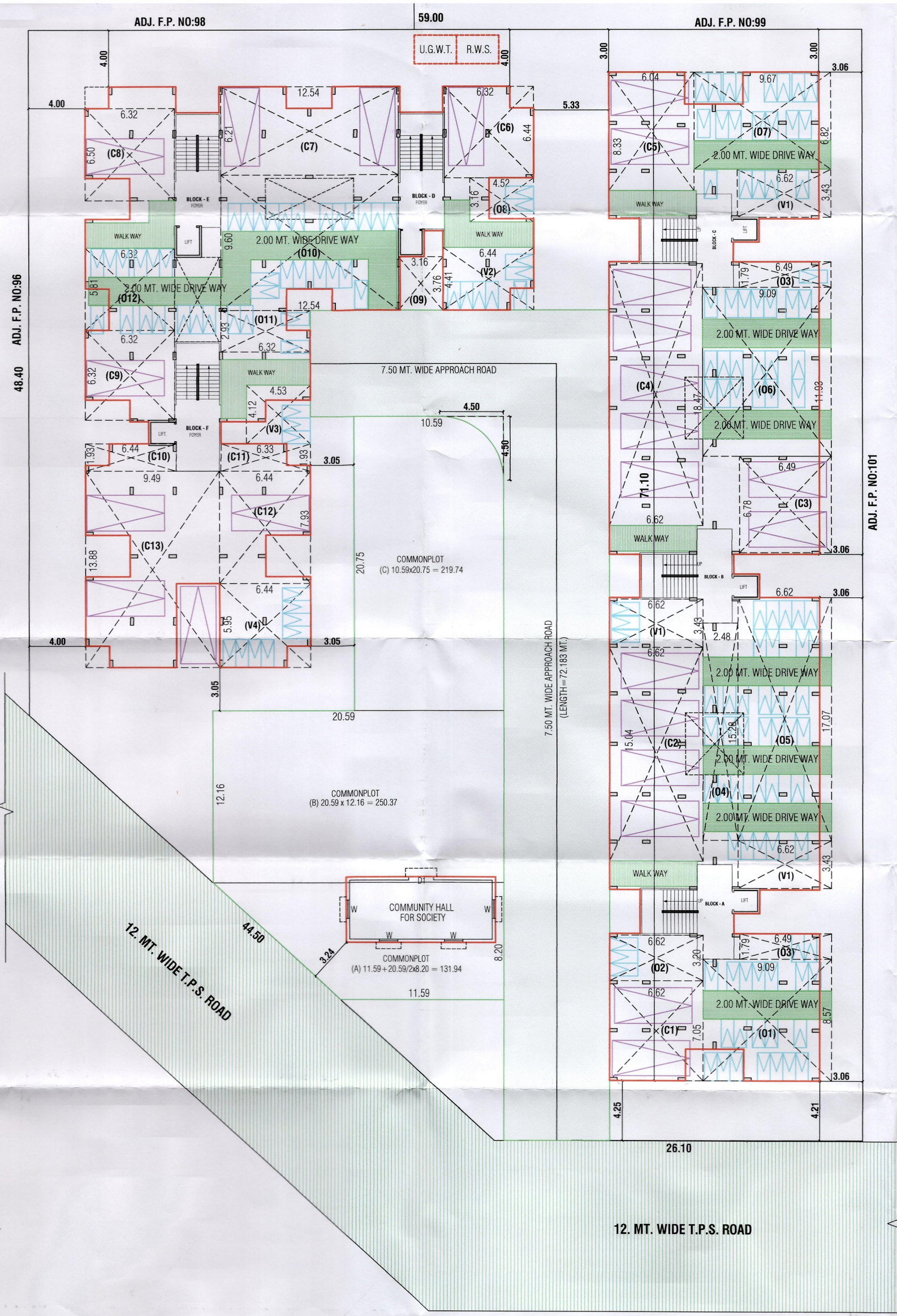
PARKING LAYOUT PLAN SCALE: 1 CM. = 2.00 MT.
