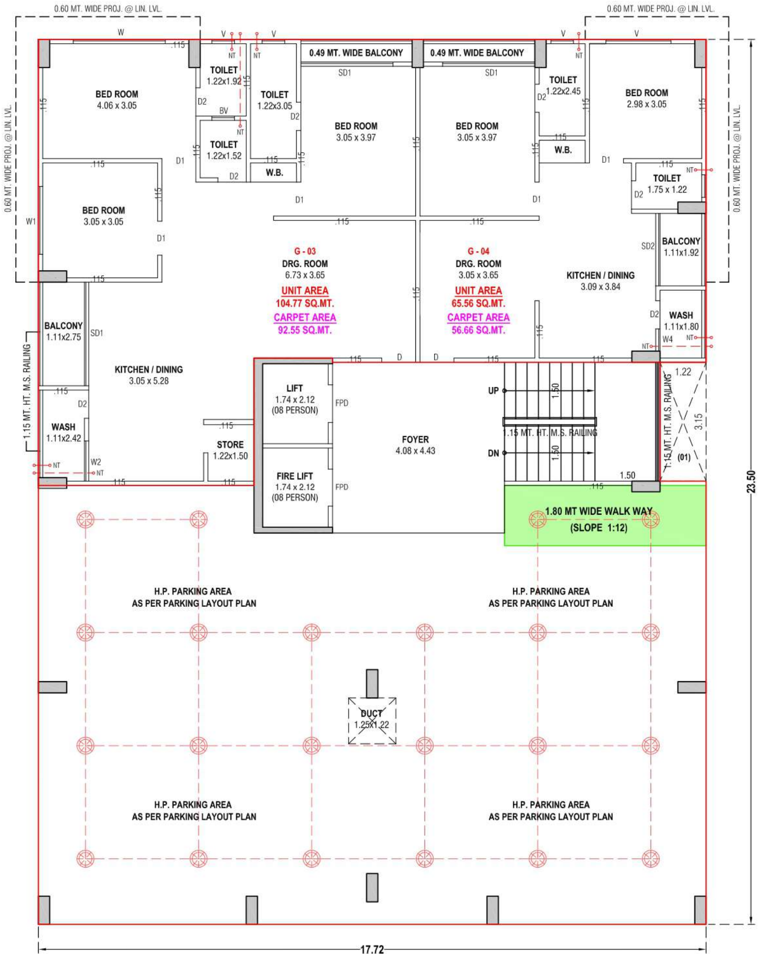
GR. FLOOR PLAN
