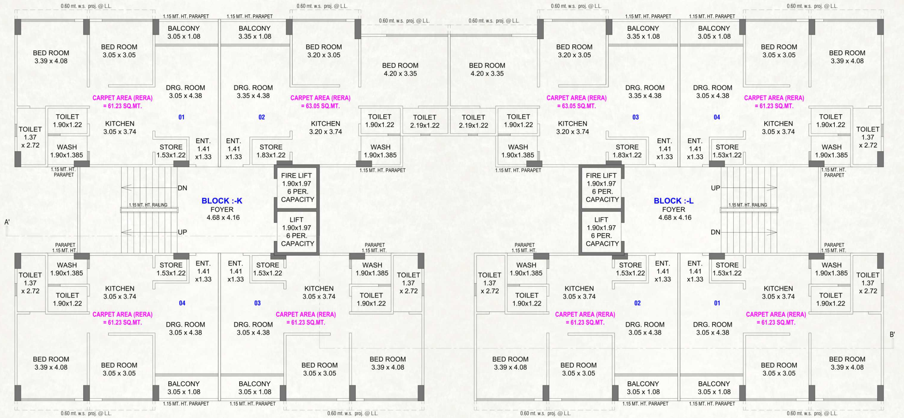
(BLOCK :- K+L) TYPICAL FLOOR PLAN
