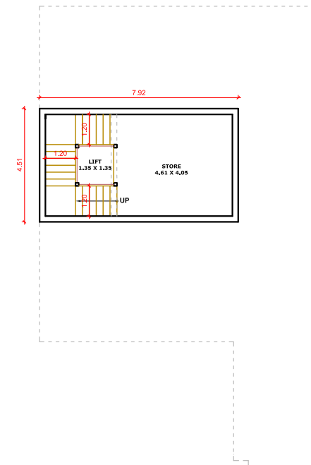
BASEMENT FLOOR PLAN
