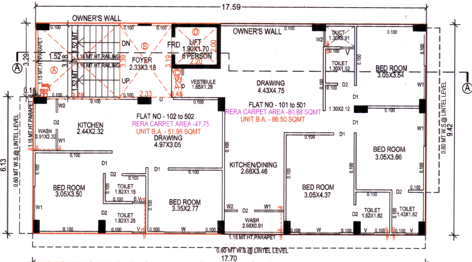
TYPICAL FLOOR PLAN ( 1st to 5th FLOOR )
