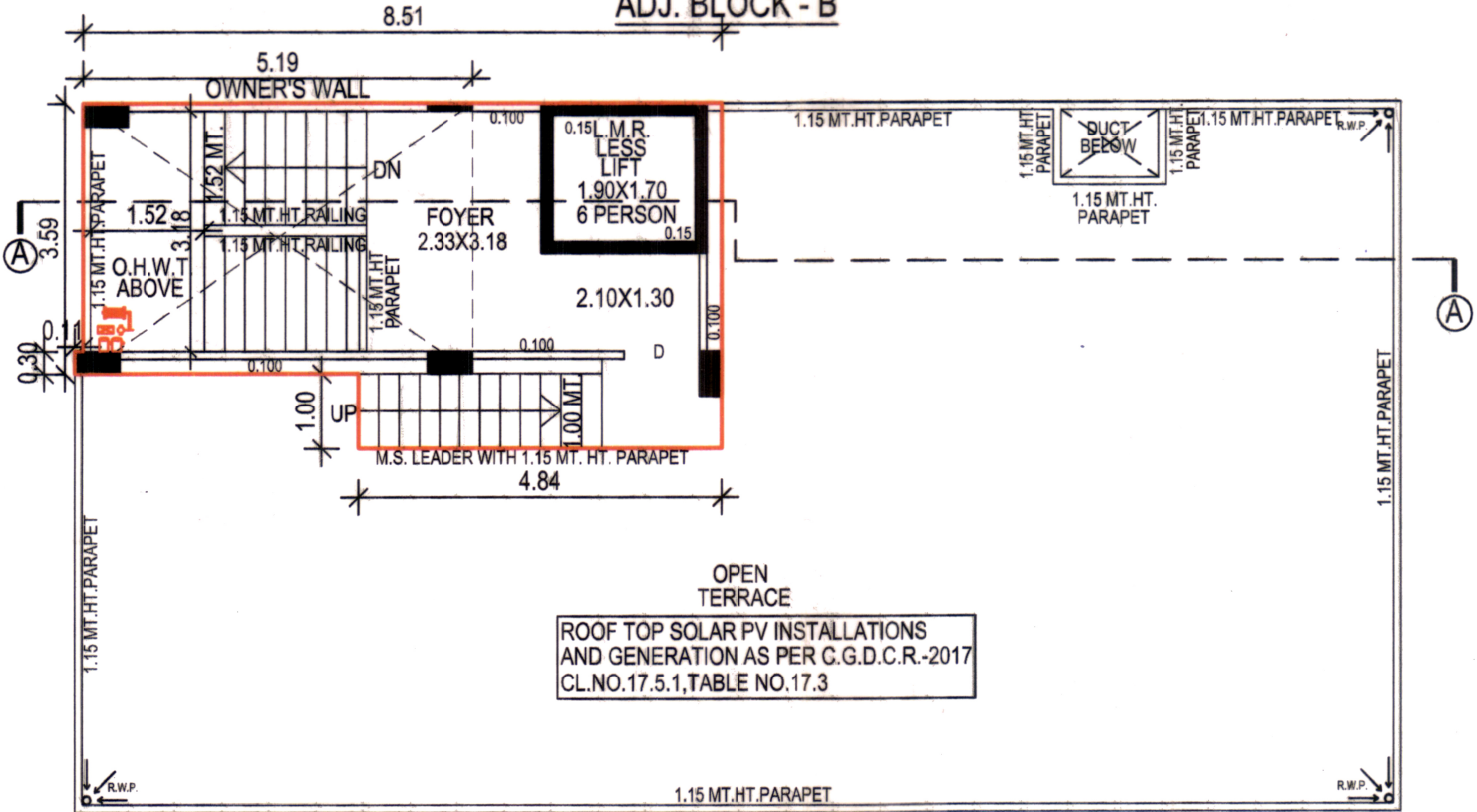
TERRACE PLAN
