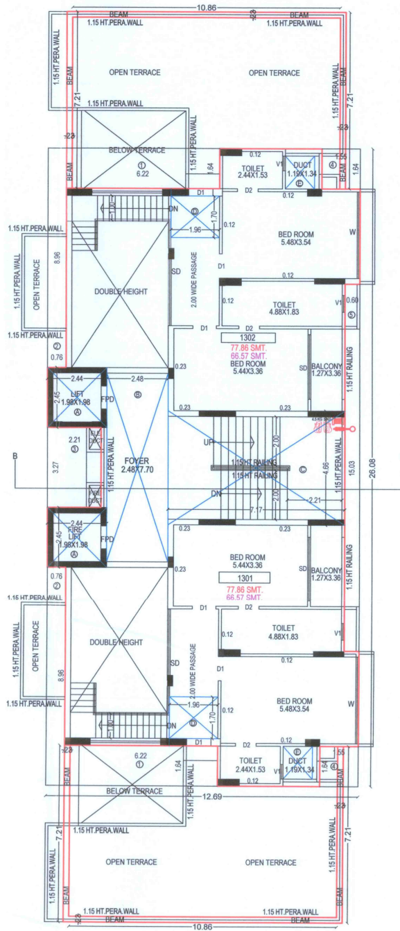
13TH FLOOR PLAN
