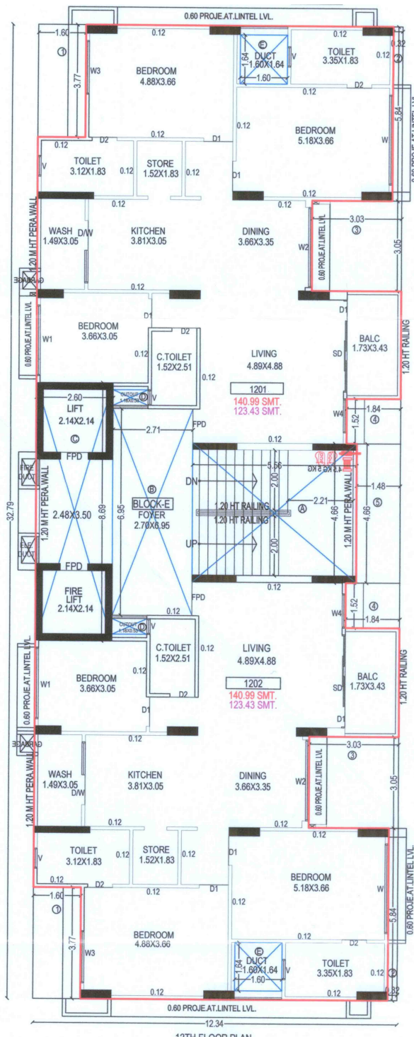
12TH FLOOR PLAN
