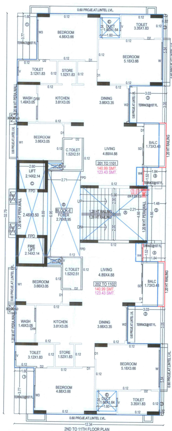
2ND TO 11TH FLOOR PLAN
