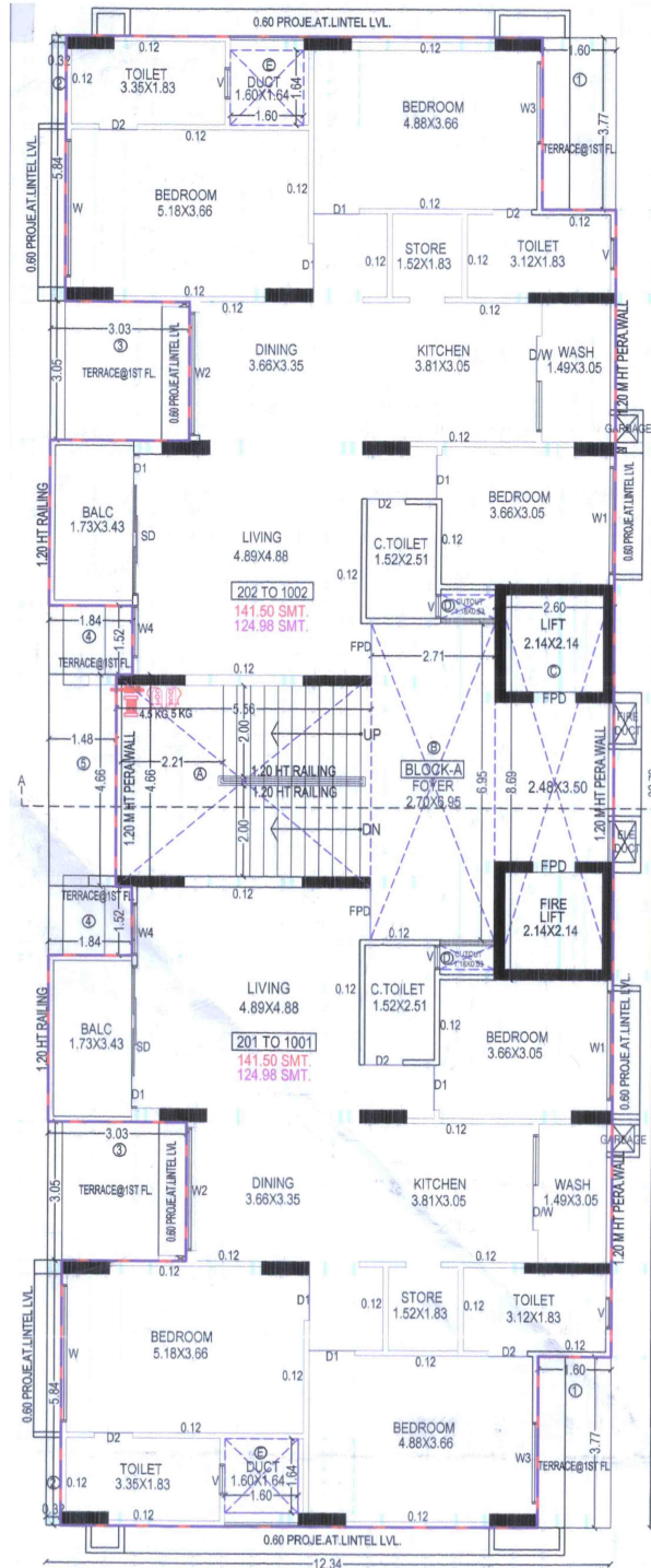
2ND TO 10TH FLOOR PLAN
