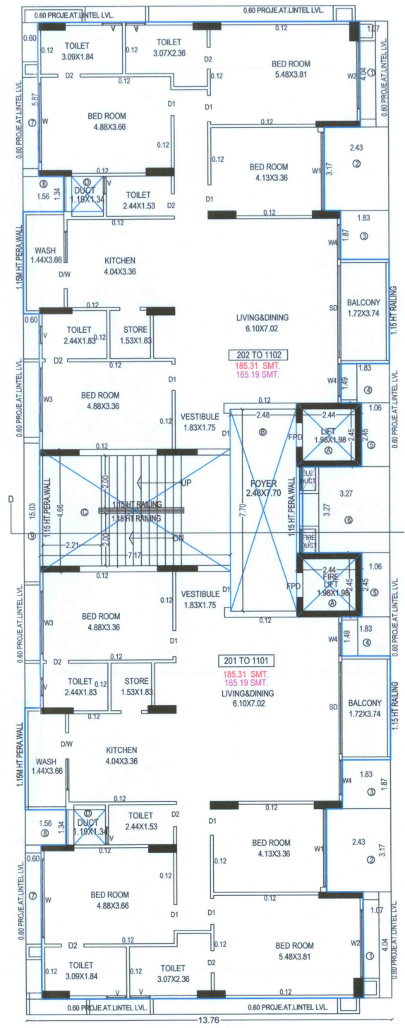
2ND TO 11TH FLOOR PLAN
