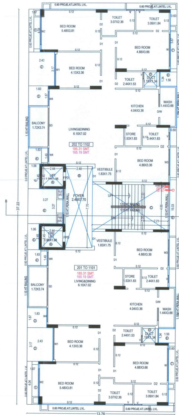
2ND TO 11TH FLOOR PLAN
