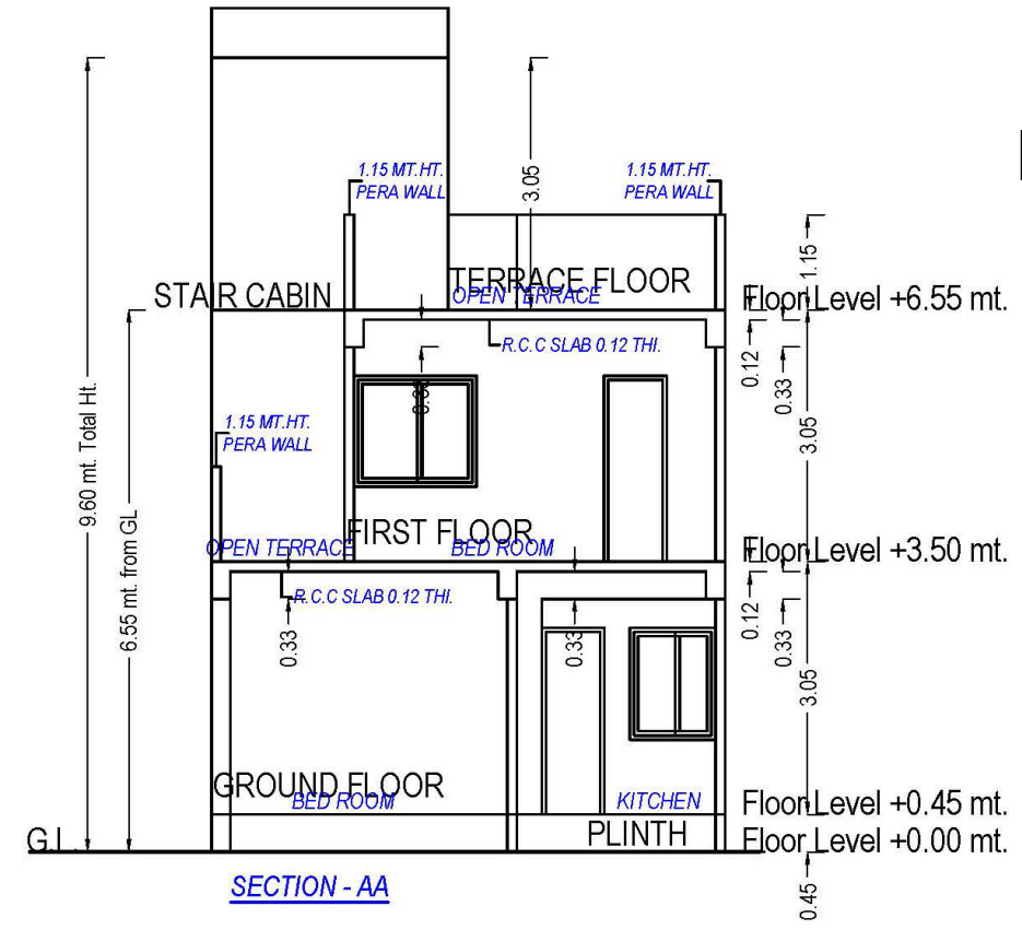
SECTION
