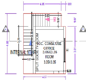
GROUND FLOOR PLAN (Proposed) (SCALE 1:100) Society Room (Building)
