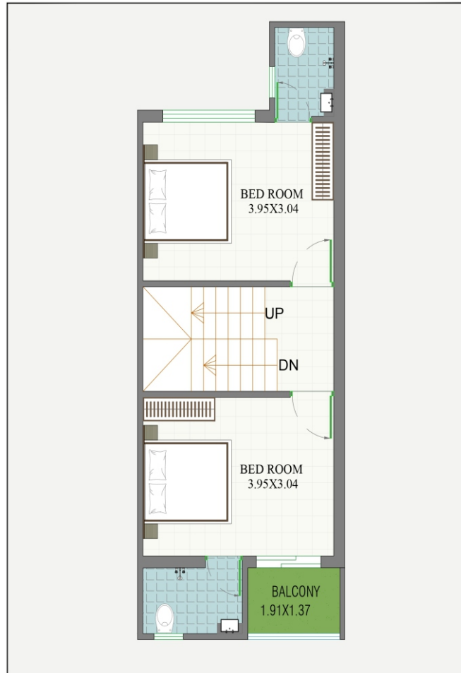
RAVI ROYALS 1ST FLOOR PLAN UNIT NO.= 41 BLOCK-C ARCHITECT CAPITAL CONSULTANCY SERVICES 504, 505, 506, GRADY, M. G. ROAD, NHOL, Ahmedabad. Email: rccs@rccs@gmail.com
