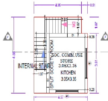
FIRST FLOOR PLAN (Proposed) (SCALE 1:100) Society Room (Building)
