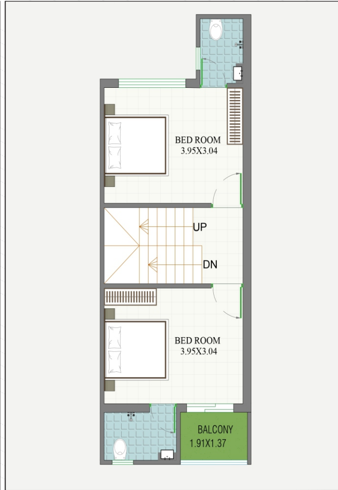
1ST FLOOR PLAN UNIT NO.= 33 BLOCK-C
