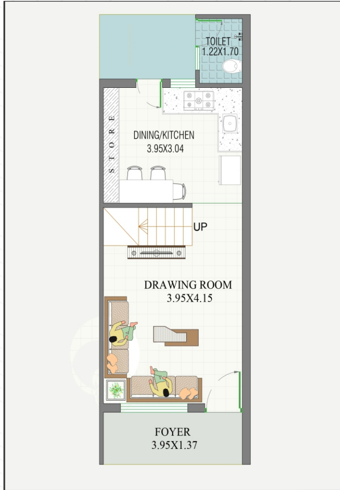
GROUND FLOOR PLAN UNIT NO.= 33 BLOCK-C
