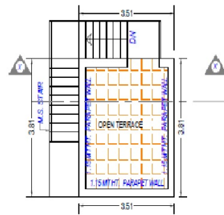
TERRACE FLOOR PLAN (SCALE 1:100) Society Room (Building)
