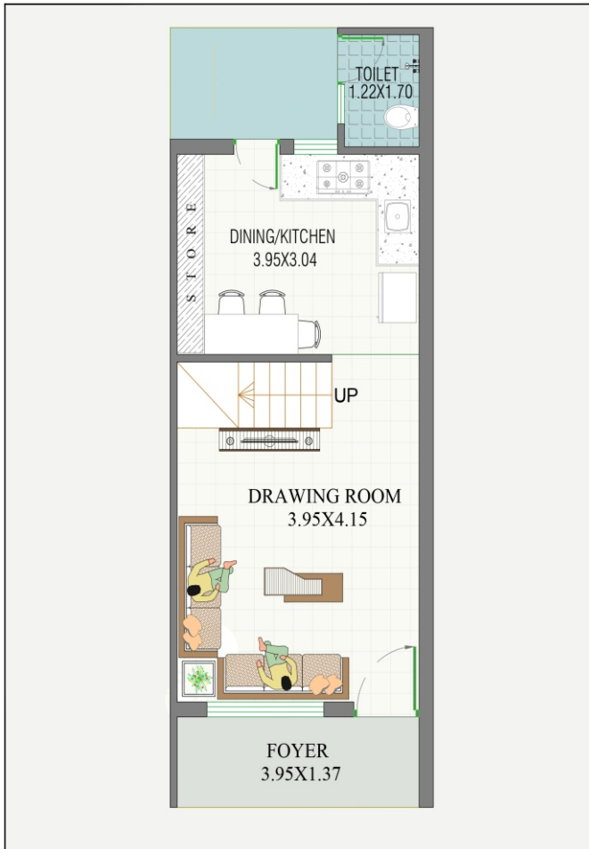
RAVI ROYALS GROUND FLOOR PLAN UNIT NO.= 26,28,30 BLOCK-C ARCHITECT CAPITAL CONSULTANCY SERVICES S 004,505,506, GRADUITY, M.G. ROAD, NHOL, Ahmedabad. Email:ccsarch@gmail.com
