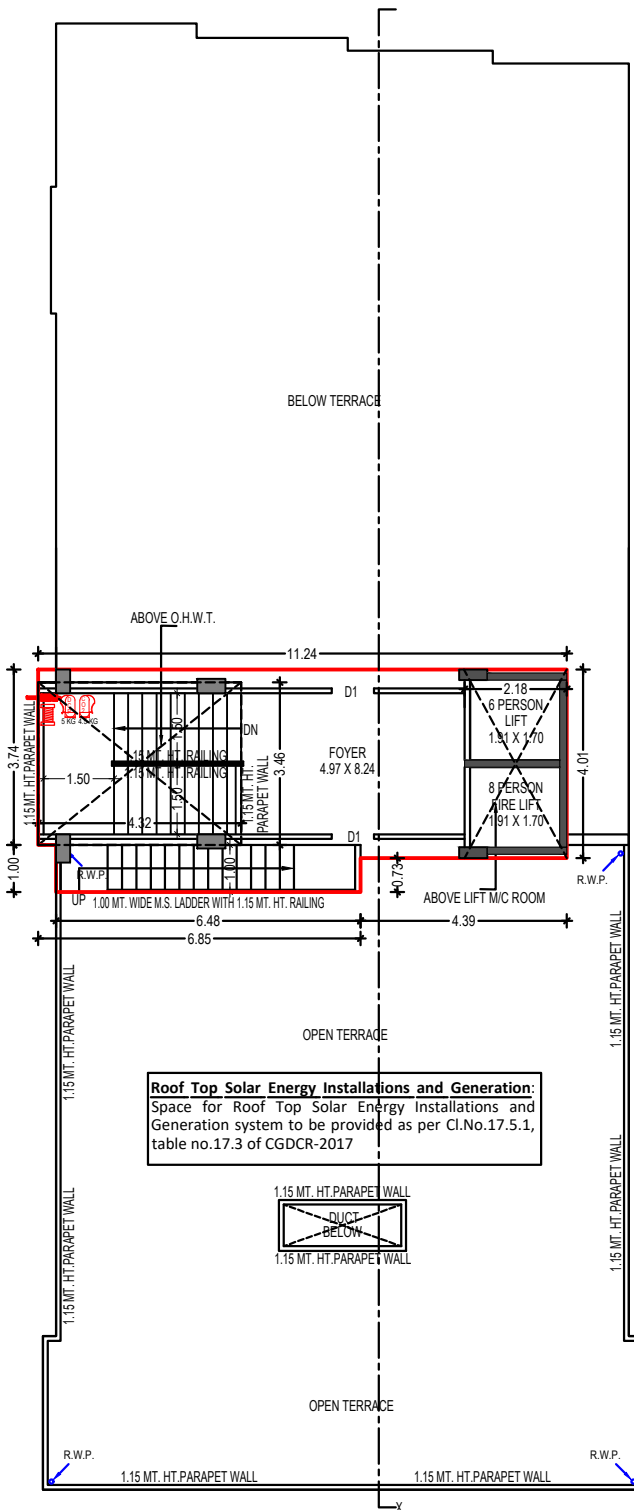
OPEN TERRACE FLOOR PLAN WITH STAIR CABIN, L.M.R. & O.H.W.T.
