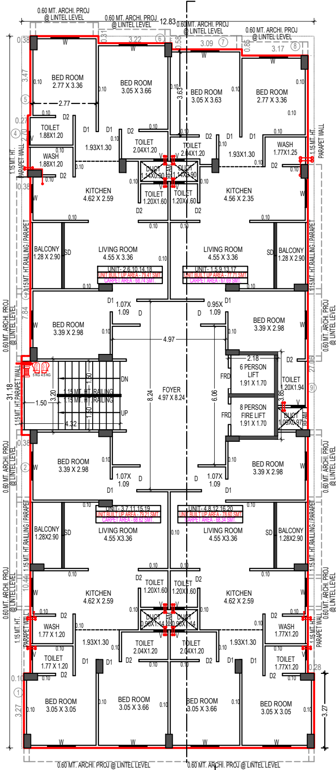
TYPICAL FLOOR (1ST TO 5TH FLOOR) PLAN
