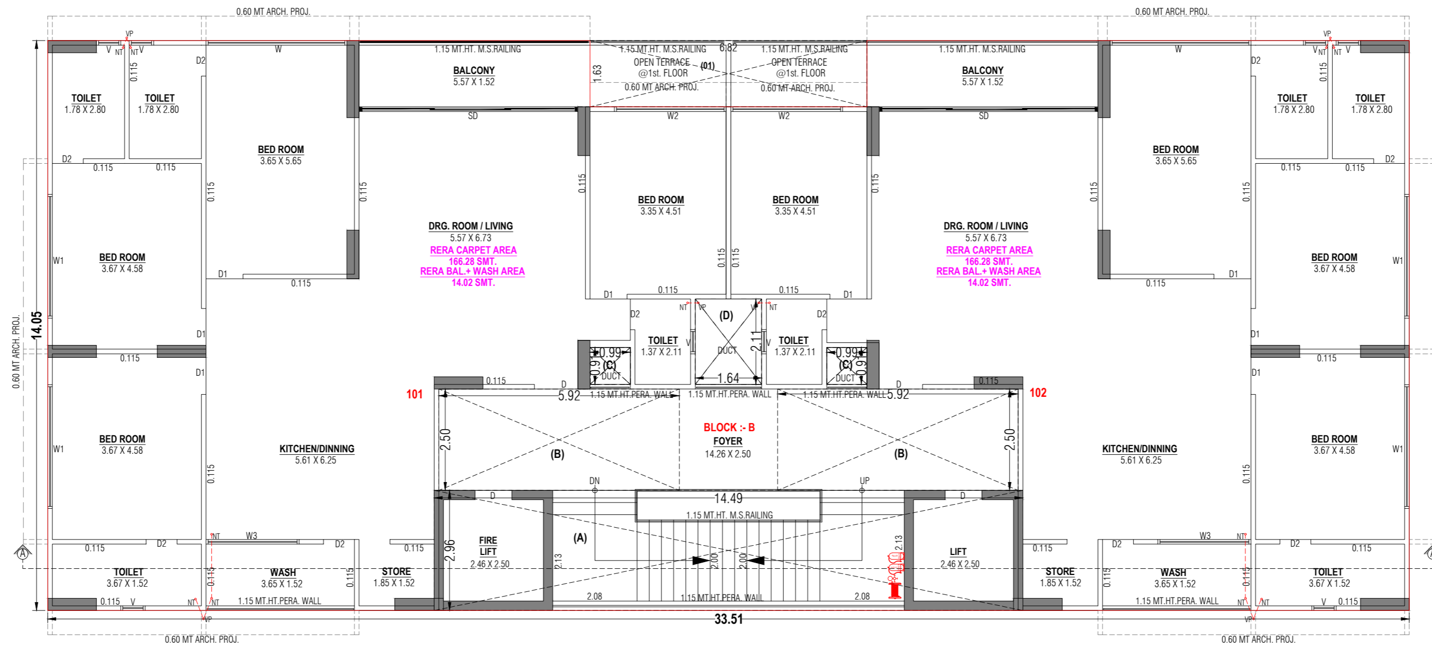
1st. FLOOR PLAN
