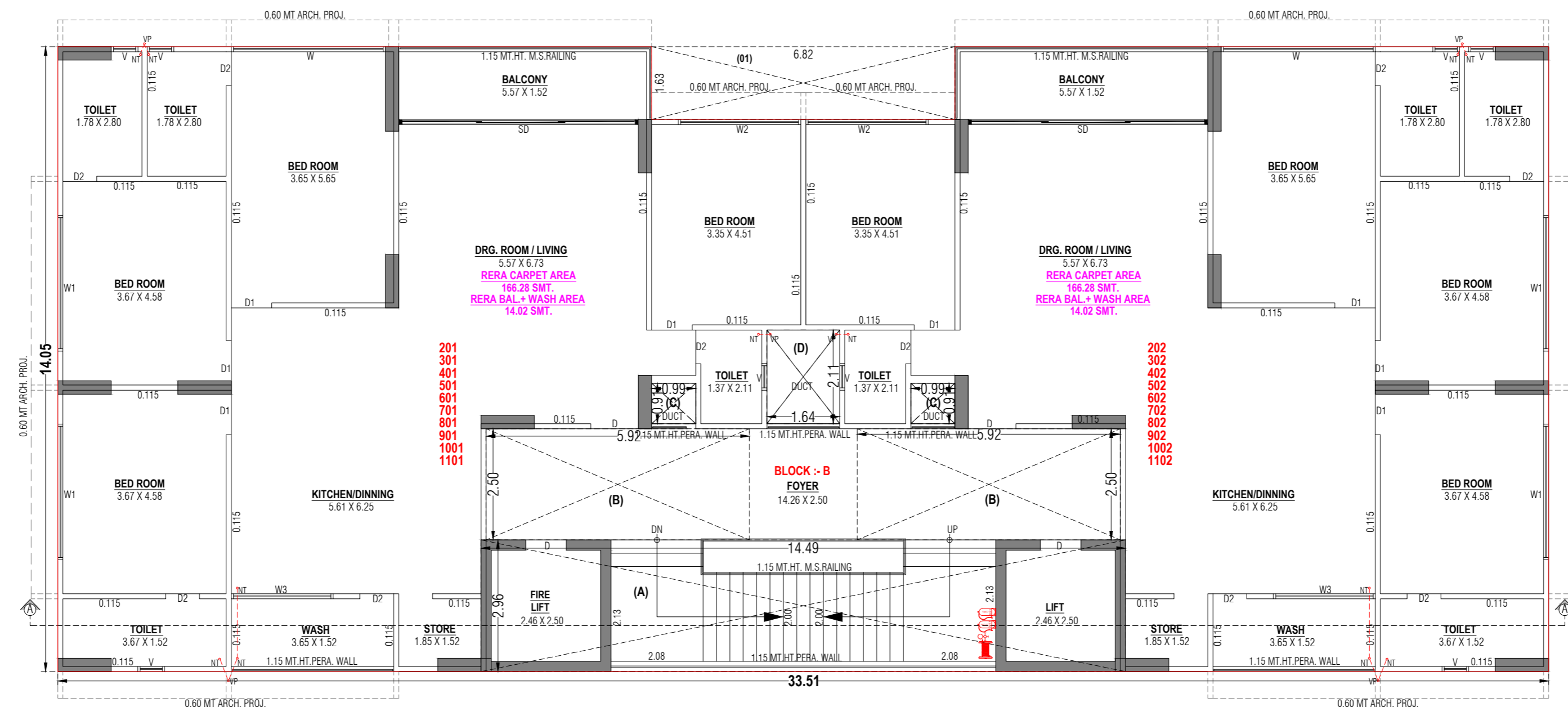
2nd to 11th. FLOOR PLAN
