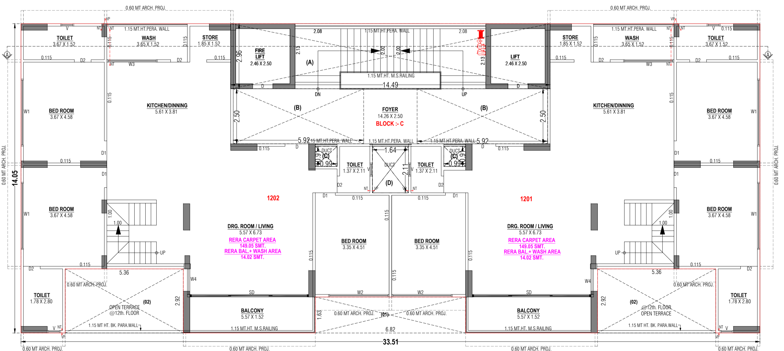
12th. FLOOR PLAN
