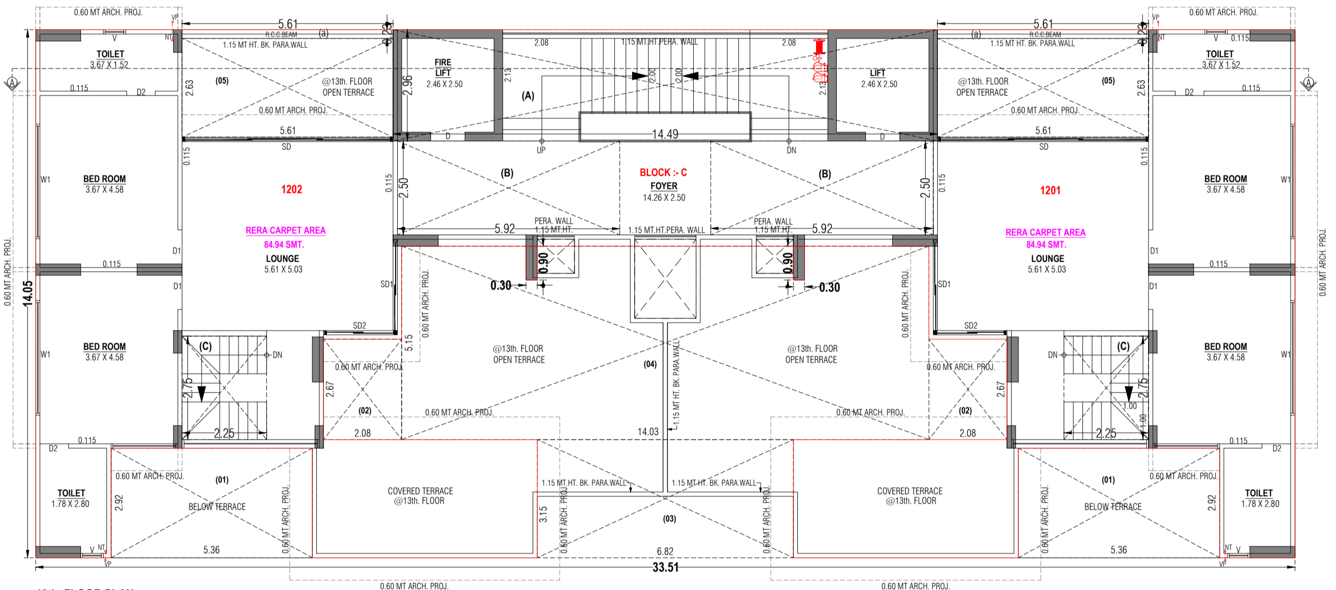
13th. FLOOR PLAN
