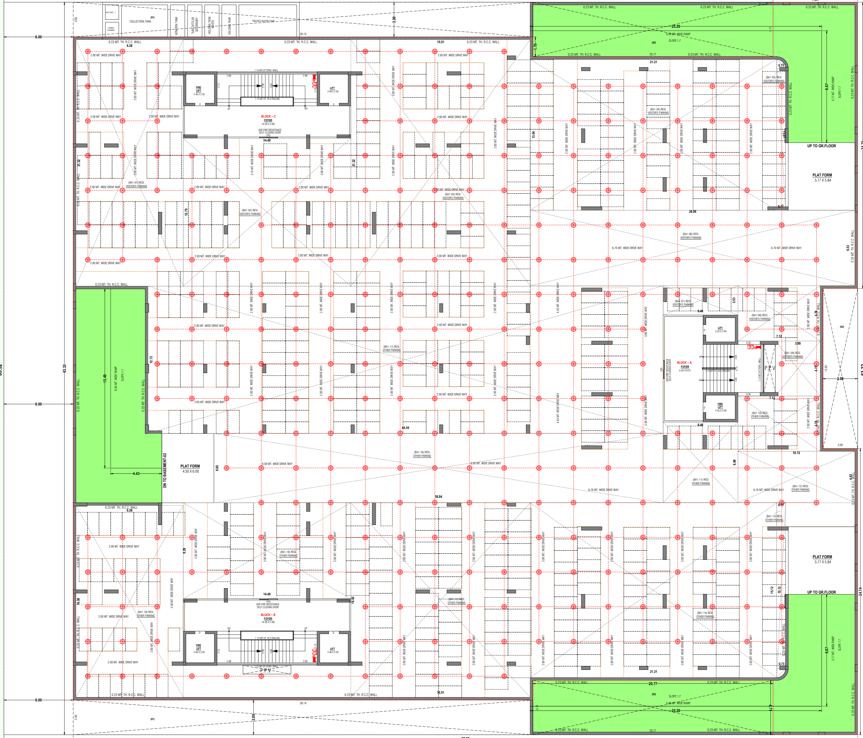
BASEMENT-01 PLAN
