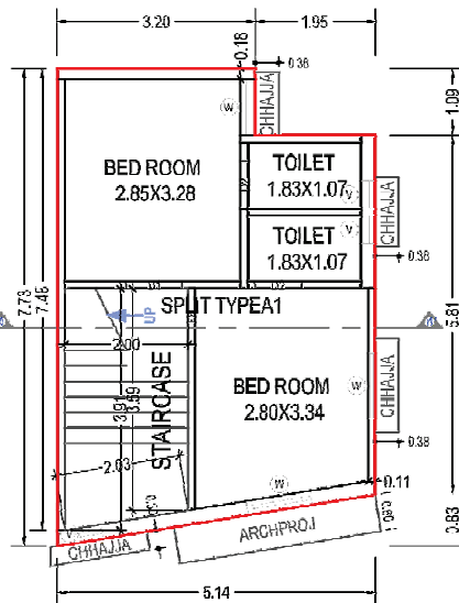
FIRST FLOOR PLAN (Proposed) (SCALE 1:100)
