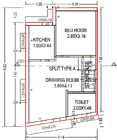
GROUND FLOOR PLAN (Proposed) (SCALE 1:100)
