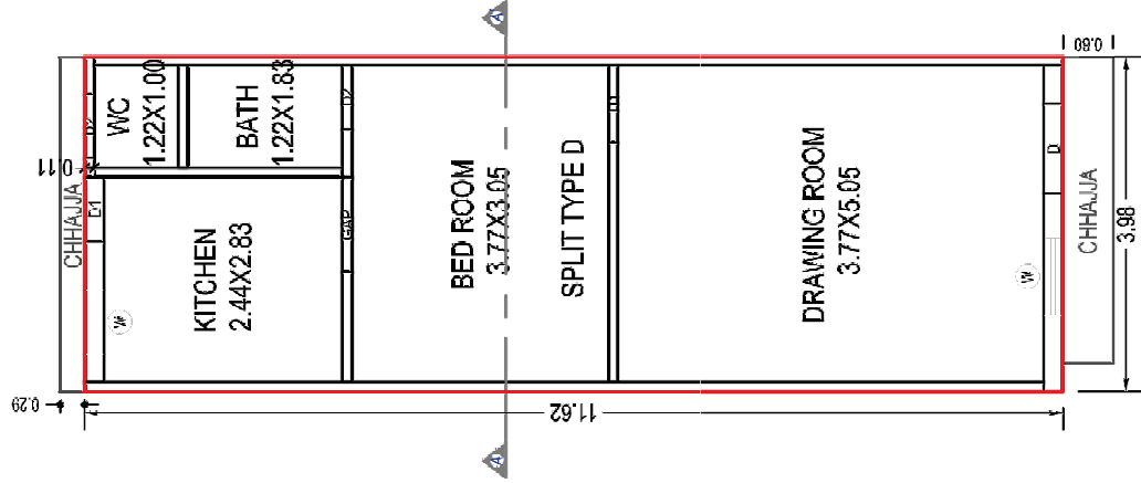
GROUND FLOOR PLAN (Proposed) (SCALE 1:100)
