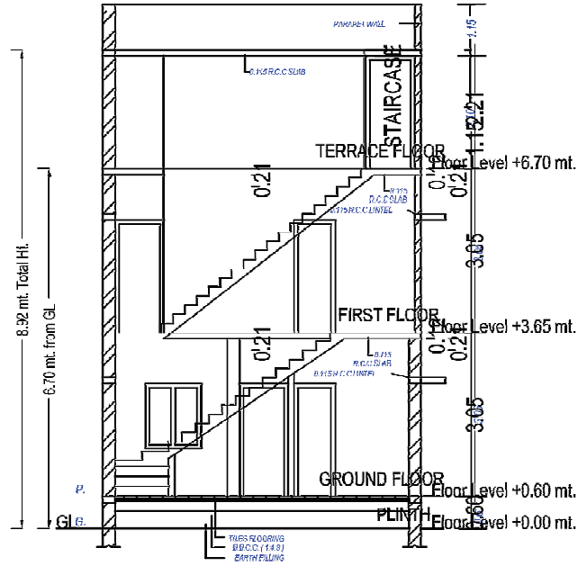
SECTION
