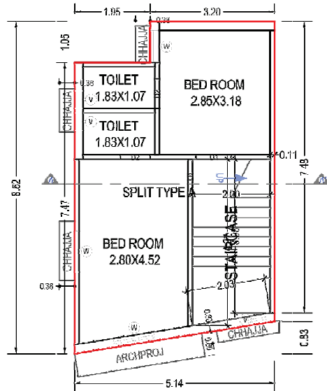
FIRST FLOOR PLAN (Proposed) (SCALE 1:100)
