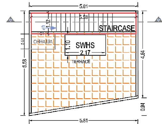
TERRACE FLOOR PLAN (SCALE 1:100)
