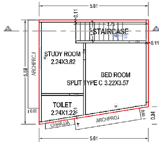
FIRST FLOOR PLAN (Proposed) (SCALE 1:100)
