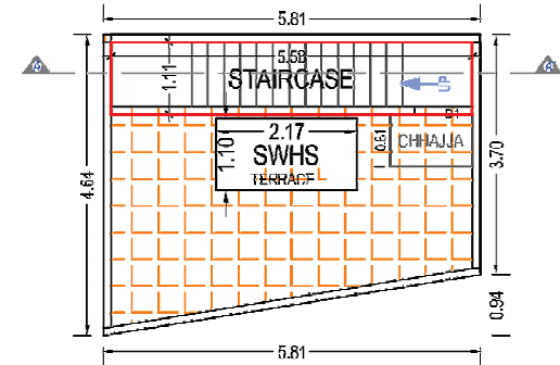
TERRACE FLOOR PLAN (SCALE 1:100)
