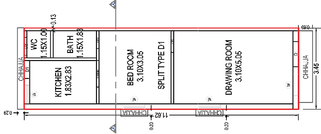
GROUND FLOOR PLAN (Proposed) (SCALE 1:100)
