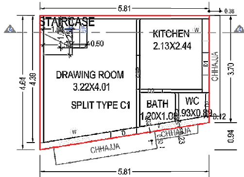
GROUND FLOOR PLAN (Proposed) (SCALE 1:100)
