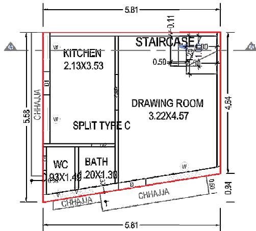
GROUND FLOOR PLAN (Proposed) (SCALE 1:100)
