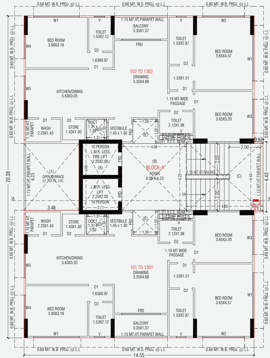
2nd to 13th Floor Plan And Carpet Area Calculation
