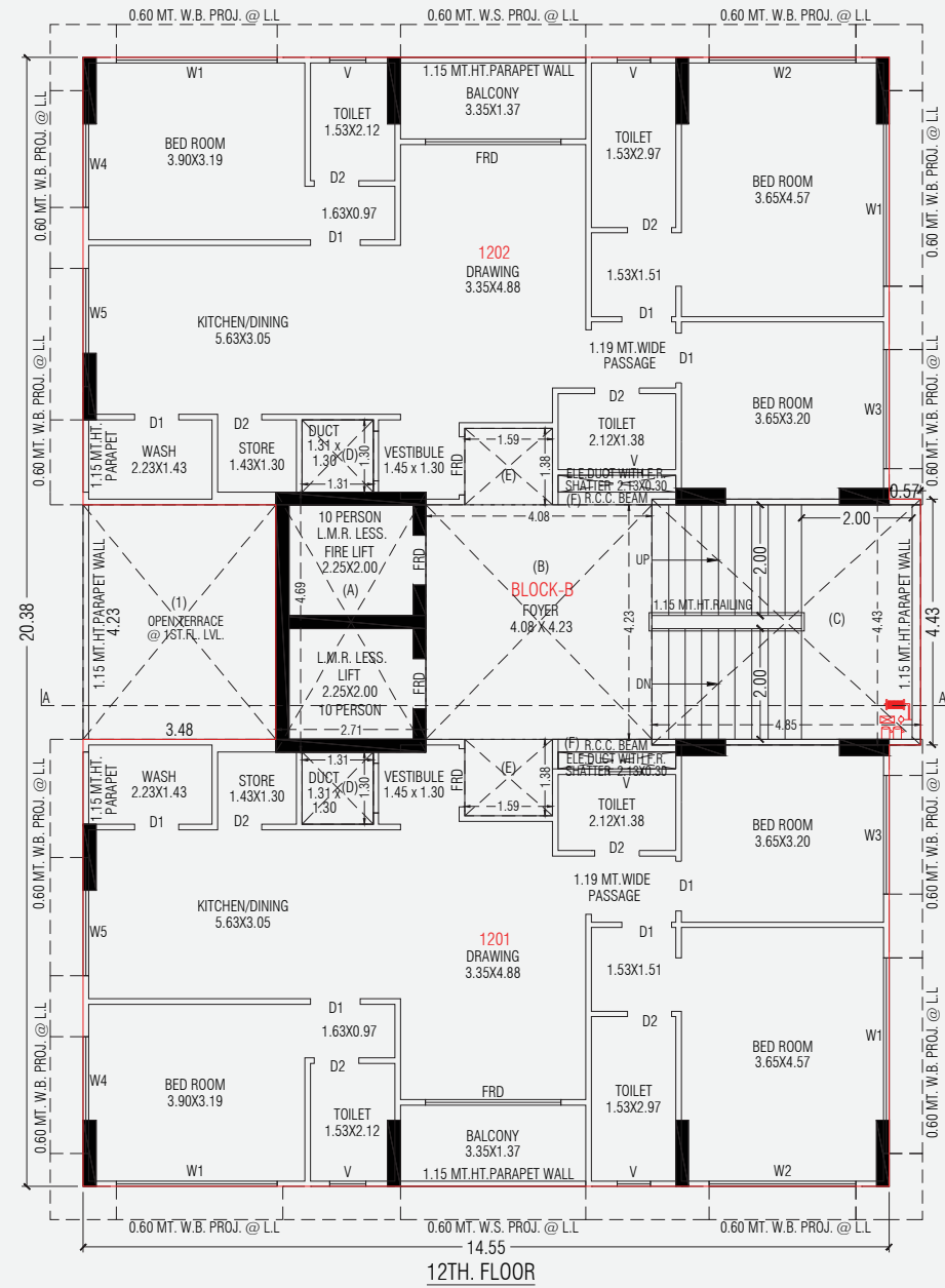
12th Floor Plan And Carpet Area Calculation
