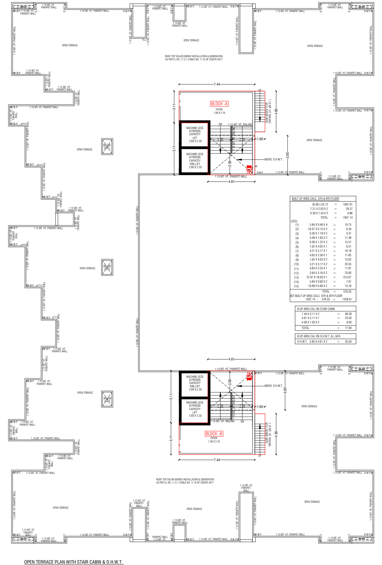
OPEN TERRACE PLAN WITH STAIR CABIN & O.H.W.T.
