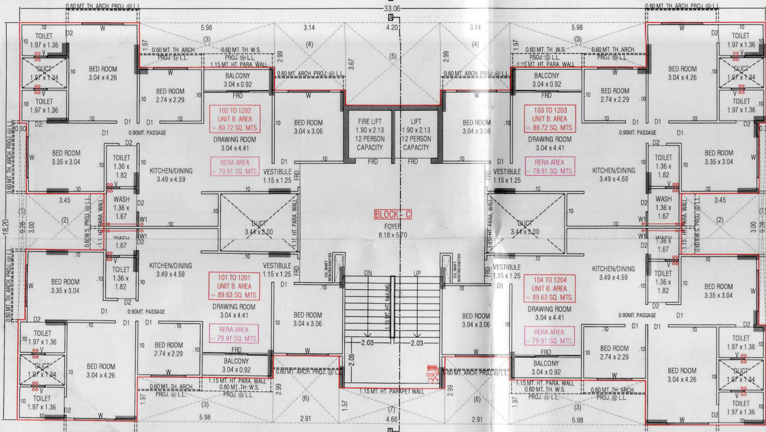
TYPICAL FLOOR PLAN ( 2ND TO 12TH FLOOR PLAN )
