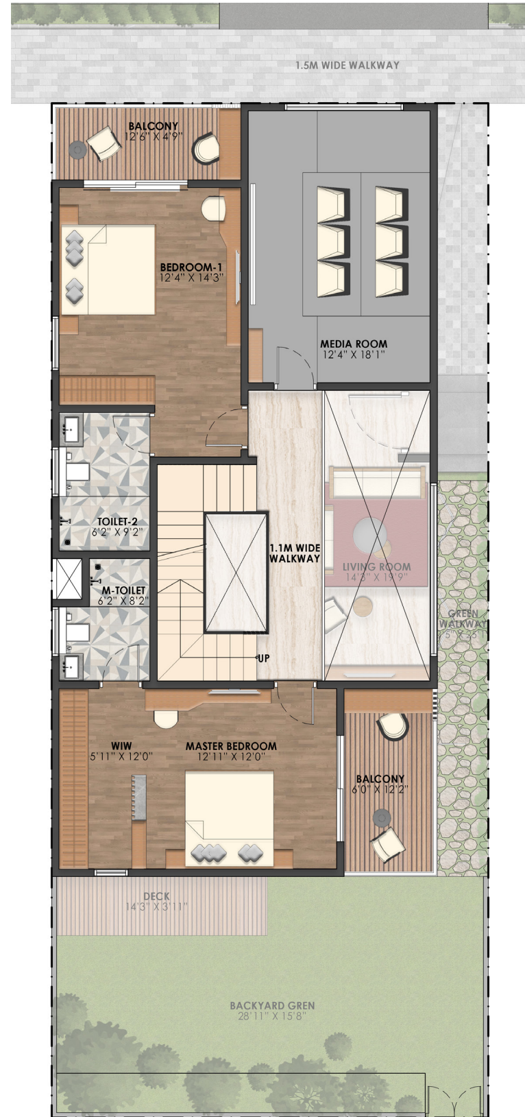
FIRST FLOOR
