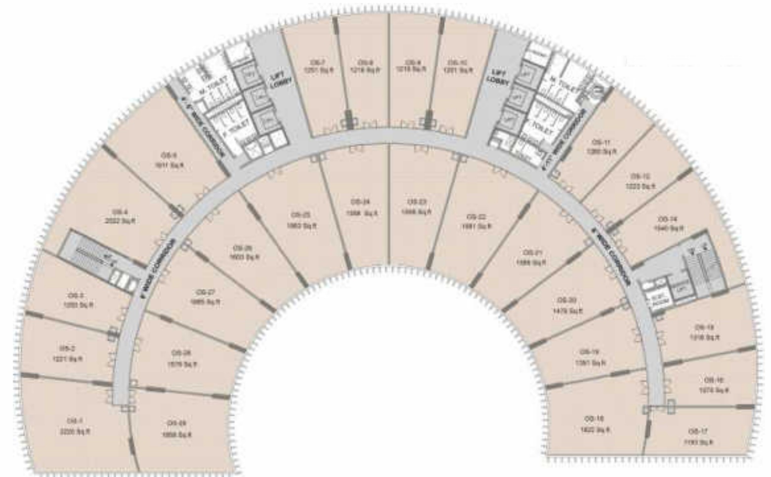
SECOND, THIRD, FOURTH & SIXTH TYPICAL FLOOR PLAN
