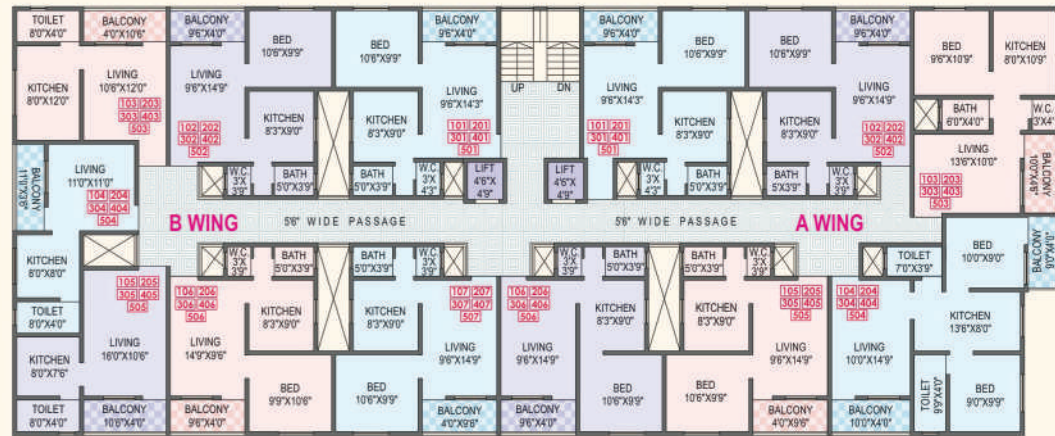
FIRST, SECOND, THIRD, FOURTH & FIFTH FLOOR PLAN
