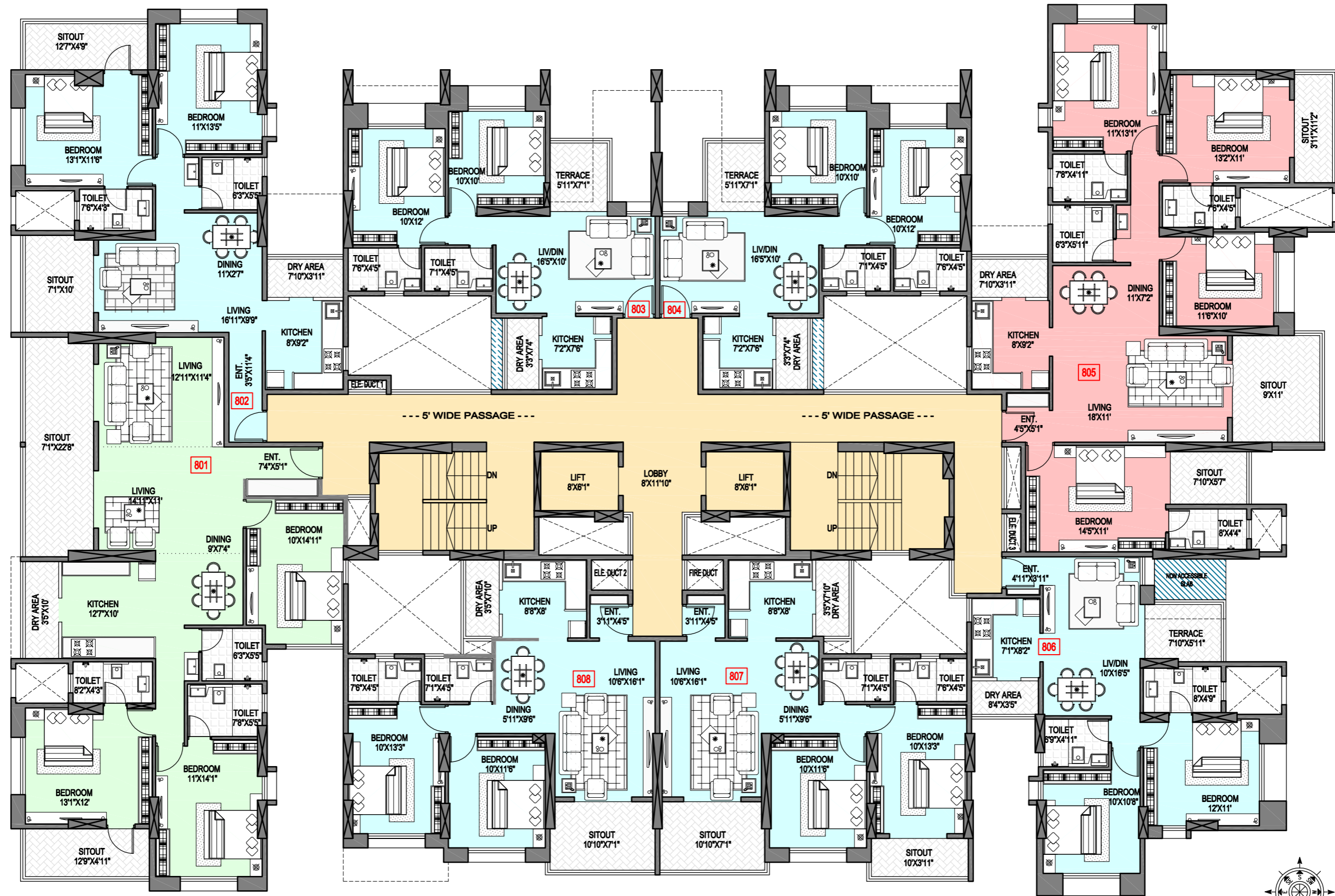
8TH FLOOR PLAN
