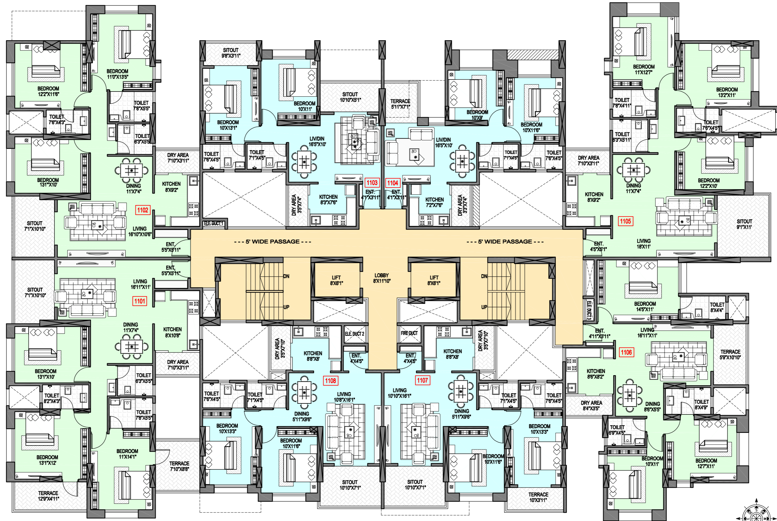
11TH FLOOR PLAN
