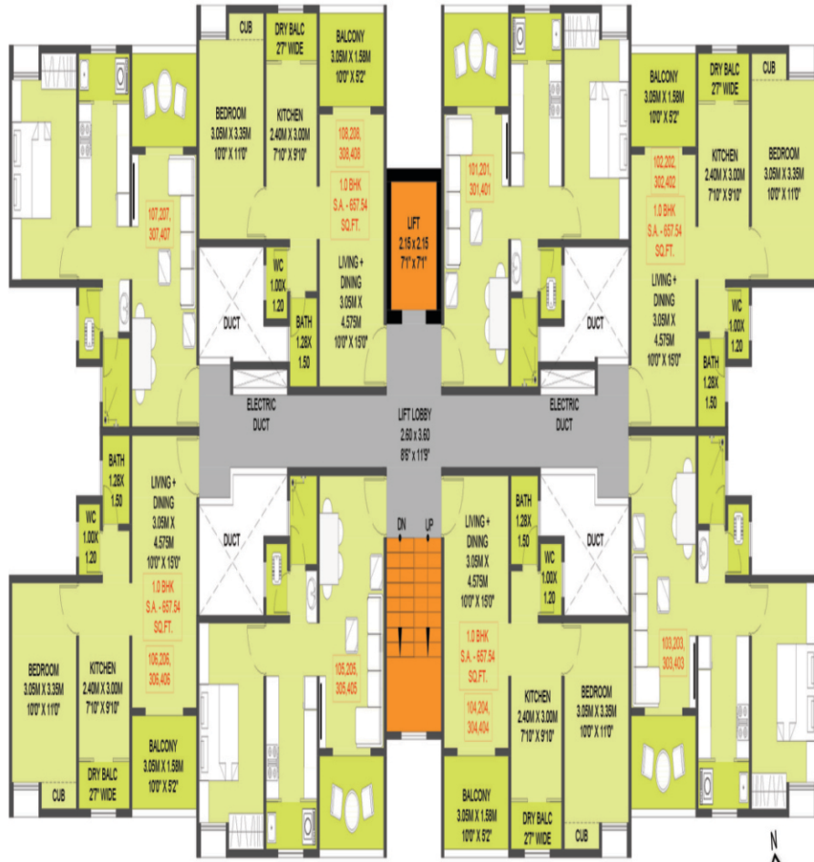
TYPICAL FLOOR PLAN - 1ST, 2ND, 3RD, 4TH
