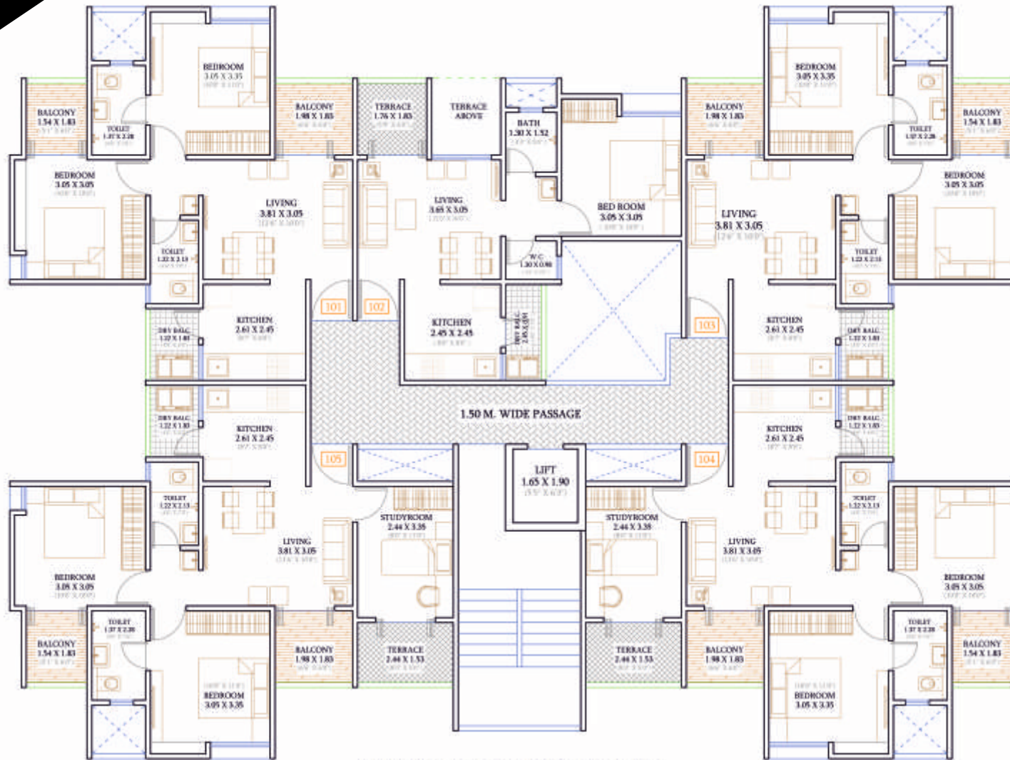
TYPICAL FLOOR PLAN ( 1st, 3rd & 5th Floor )
