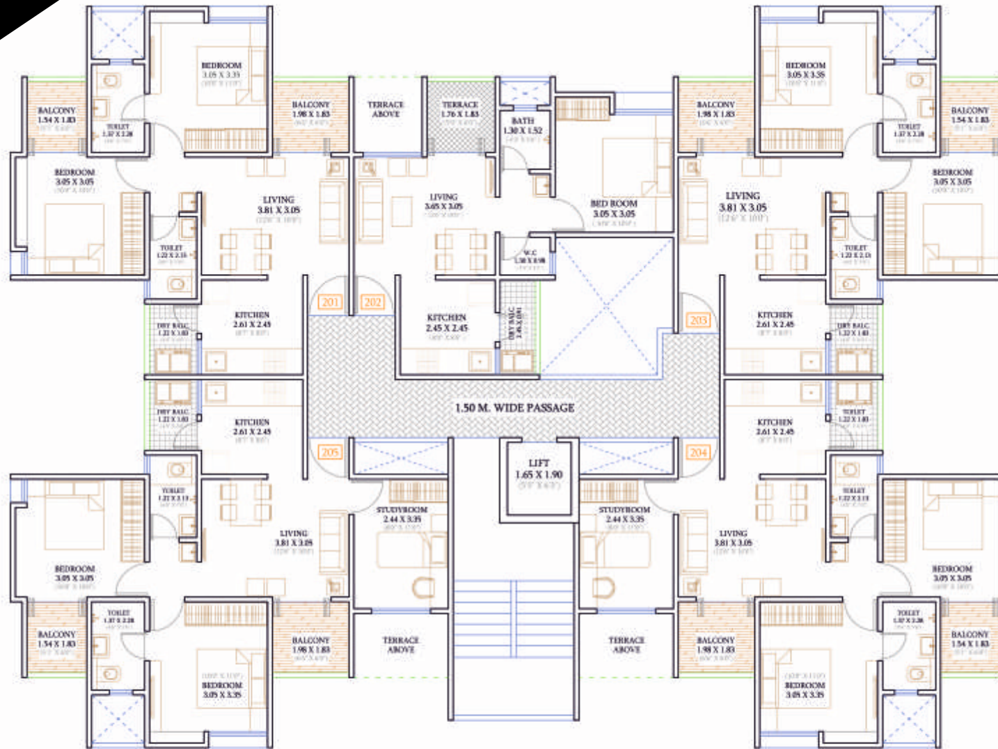
TYPICAL FLOOR PLAN ( 2nd & 4th Floor )
